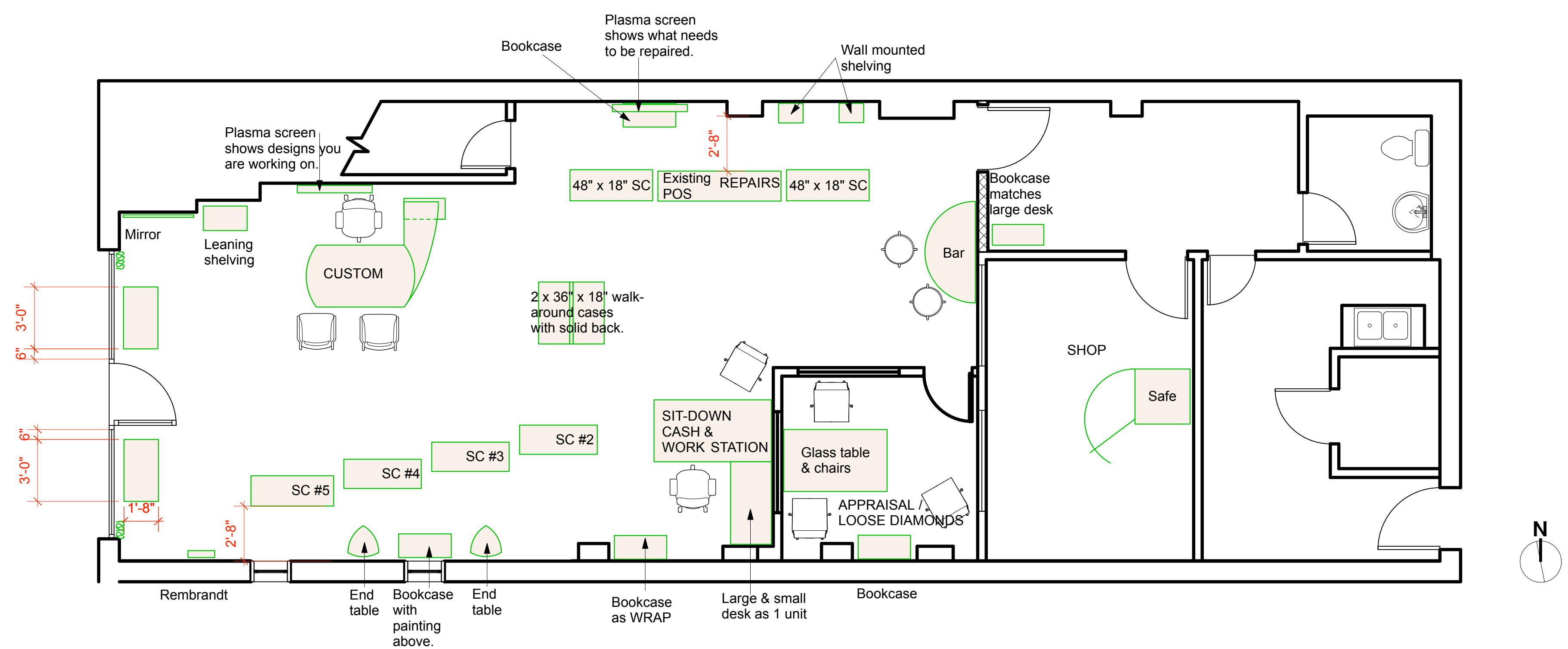
1 FIXTURE LAYOUT A Scale: 1/4" = 1'-0"
