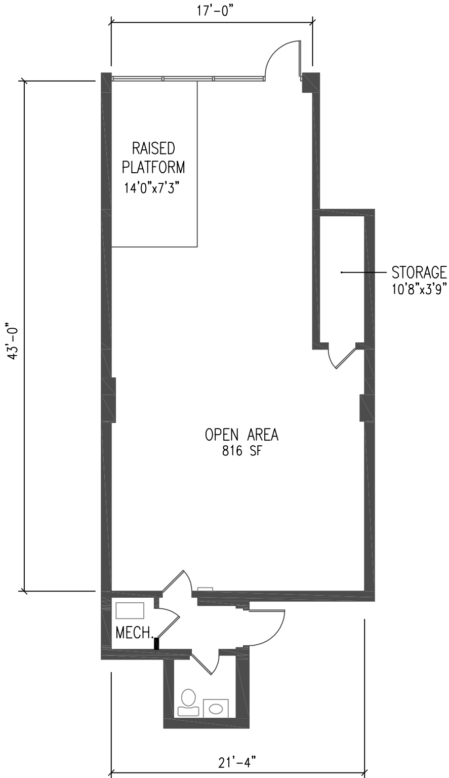
FLOOR PLAN
